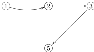
Figura 3: Camino P = (1, 2, 3, 5) .
